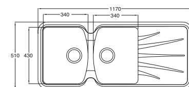
CUTOUT 1146 x 486mm Corner radiuses 58mm
