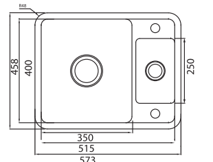
CUTOUT 521 x 406mm Corner radiuses 27mm
