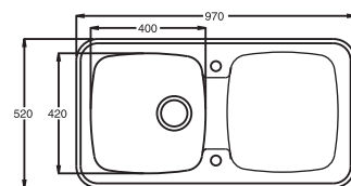
CUTOUT* 930 x 480mm Corner radiuses 55mm
