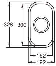
CUTOUT 162 x 300mm Corner radiuses 60mm
