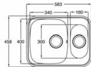
CUTOUT 563 x 438mm Corner radiuses 82mm
