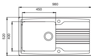
CUTOUT* 956 x 496mm
