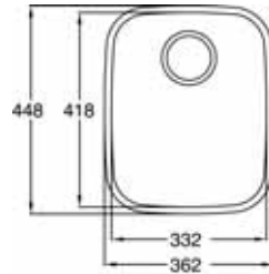
CUTOUT 332 x 418mm Corner radiuses 70mm
