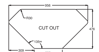
NB: This model will require a 750mm worktop when fitting to a corner unit.
