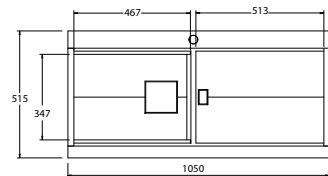
CUTOUT 1030 x 495mm
