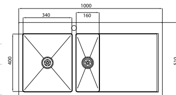
CUTOUT 980 x 490mm
