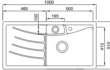
CUTOUT* 970 x 480mm
