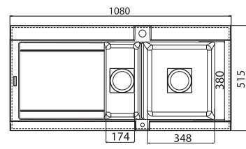
CUTOUT 1056 x 491mm
