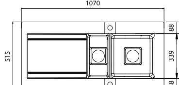
CUTOUT* 1046 x 491mm
