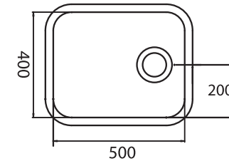
CUTOUT 495 x 395mm Corner radiuses 68mm
