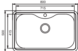
CUTOUT 780 x 480mm Corner radiuses 50mm
