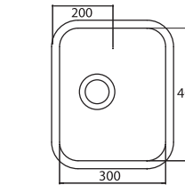
CUTOUT 295 x 395mm Corner radiuses 68mm
