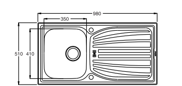
CUTOUT 960 x 490mm
