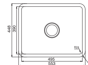
CUTOUT 501 x 396mm Corner radiuses 27mm
