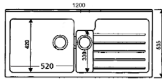
CUTOUT* 1176 x 511mm
