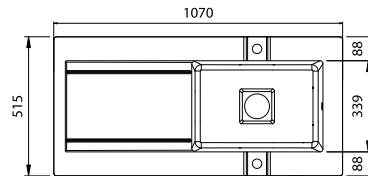
CUTOUT* 1046 x 491mm
