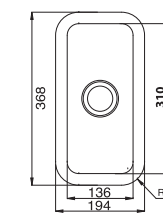
CUTOUT 142 x 316mm Corner radiuses 27mm
