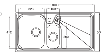
CUTOUT 980 x 480mm
