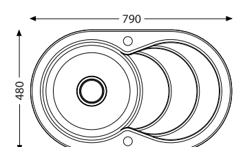
CUTOUT 766 x 456mm
