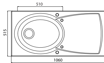
CUTOUT 1036 x 491mm
