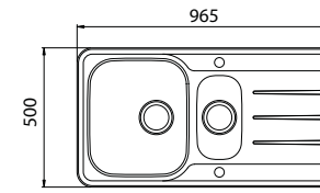
CUTOUT 945 x 480mm
