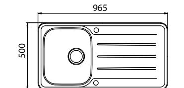
CUTOUT 945 x 480mm
