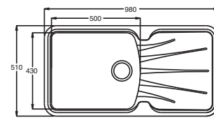
CUTOUT 956 x 486mm Corner radiuses 58mm
