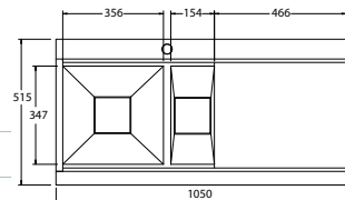
CUTOUT 1030 x 495mm
