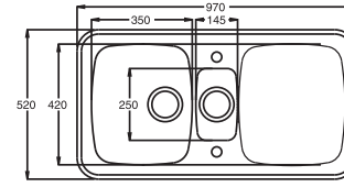
CUTOUT* 930 x 480mm Corner radiuses 55mm Minimum tap reach 120mm
