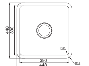
CUTOUT 396 x 396mm Corner radiuses 27mm
