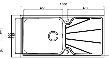
CUTOUT 980 x 480mm
