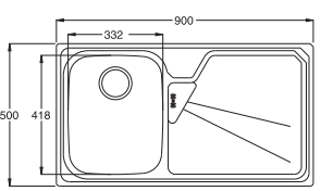
CUTOUT 880 x 480mm
