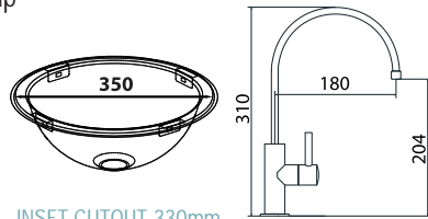
INSET CUTOUT 330mm U/M CUTOUT 290mm
