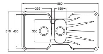
CUTOUT 956 x 486mm Corner radiuses 58mm
