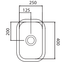
CUTOUT 245 x 395mm Corner radiuses 68mm
