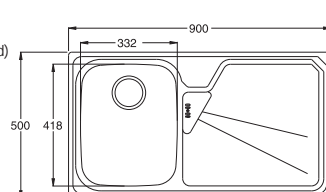
CUTOUT 884 x 484mm
