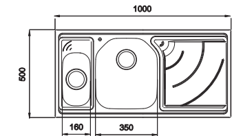
CUTOUT 980 x 480mm
