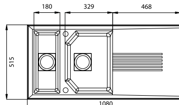
CUTOUT 1056 x 491mm
