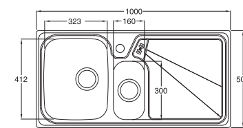
CUTOUT 976 x 476mm
