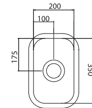
CUTOUT 195 x 345mm Corner radiuses 68mm
