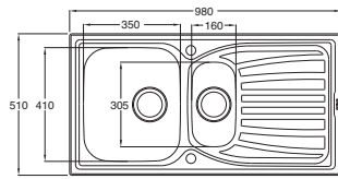
CUTOUT 960 x 490mm
