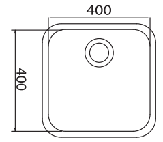
CUTOUT 395 x 395mm Corner radiuses 68mm
