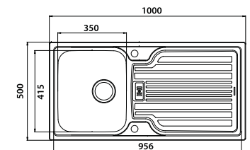
CUTOUT 980 x 480mm
